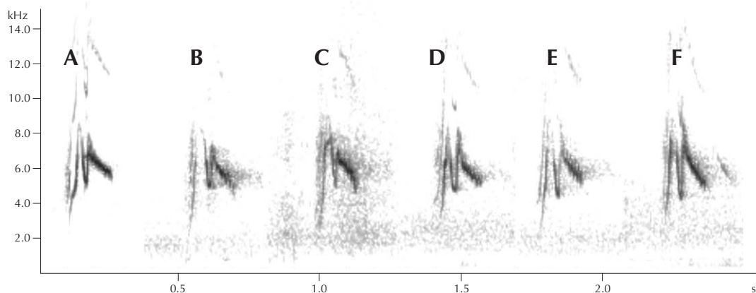
FIGURE 25 Calls of yellow wagtail / gele kwikstaart Motacilla flava sensu lato . Examples of calls with pronounced frequency dips in middle, typical, possibly even diagnostic, of breeders between Yamal/Ob river basin and Taimyr. A male, southern Yamal, Russia, 10 June 2015 (Giovanni Boano). B dark-headed male, Novy Urengoy, Russia, 8 July 2017 (Alexander Hellquist). C female, Tazovsky, Russia, 7 July 2017 (Alexander Hellquist). D dark-headed male, Norilsk, Russia, 8 July 2015 (Alexander Hellquist). E male with prominent supercilium (plate 484), Khatanga, Russia, 10 July 2015 (Alexander Hellquist). F male with weak supercilium, Khatanga, Russia, 10 July 2015 (Alexander Hellquist).
