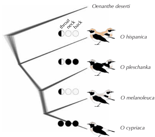
FIGURE 3 Species tree showing the phylogenetic relationships of the taxa in the Oenanthe hispanica-melano-leuca-cypriaca-pleschanka complex. Modified from Schweizer et al (2019). Desert Wheatear O. deserti was used as outgroup for the species tree reconstructions. The outgroup 'roots' the tree, a prerequisite for inferring the sequence of branching events in the 'ingroup'.
