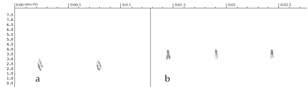
sonogram 16 Type D ('jip') Common Crossbill / Kruisbek Loxia curvirostra , alarm and chitter calls Baarn, Baarn , Utrecht ( Magnus S Robb ). a 9 March 1998 (track 36). Alarm call. b 9 March 1998 (track 37b). Chitter call
