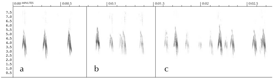
sonogram 14 Type D ('jip') Common Crossbill / Kruisbek Loxia curvirostra , flight calls, Baarn, Baarn , Utrecht, 15 March 1998 ( Magnus S Robb ). Shaped like three-pronged fork: middle and right-hand prongs more or less parallel and usually longer than left-hand prong. Apex at c 5.0-5.5 kHz higher than in Type F. Little variation encountered so far. a (track 34a). b (track 34b). c (track 34c)
