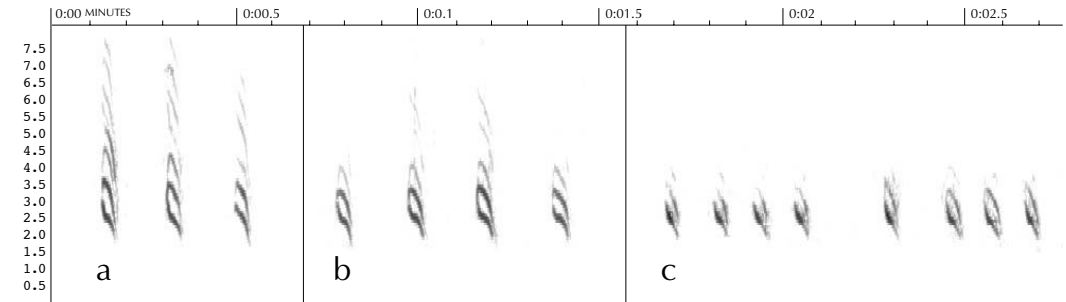
sonogram 15 Type D ('jip') Common Crossbill / Kruisbek Loxia curvirostra , excitement calls, Baarn, Baarn , Utrecht ( Magnus S Robb ). Steeply descending. Lowest and second bands differently shaped (concave and convex curves) but of roughly same duration. Third band weak but stronger than fourth. Sometimes produced in fast series. a 15 March 1998 (track 35a). b 13 March 1998 (track 35b). c 13 March 1998 (track 35c). Part of very fast series recorded at a distance. Upper bands missing due to distance
