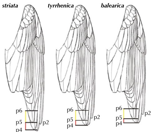
FIGURE 1 Wing-formula of Spotted Flycatcher / Grauue Vliegenvanger Muscicapa striata , Tyrrhenian Flycatcher / Tyrrhense Vliegenvanger M tyrrhenica tyrrhenica and Balearic Flycatcher / Balearische Vliegenvanger M t balearica (Lorenzo Starnini). Note longer distance between tips of p4 and p5 (red) and tips of p5 and p6 (yellow) in Spotted (wing-tip = p3) compared with both Tyrrhenian and Balearic, in which, particularly in latter, distance between these primary tips is shorter. Differences in position of p2 relative to p3 and p5 were already described by Viganò et al (2019). 332 Spotted Flycatcher / Grauue Vliegenvanger Muscicapa striata , adult, Falsterbo, Skåne, Sweden, 22 August 2015 (Marc Illa). Note long distance between tips of p4 and p5 and tips of p5 and p6, with wing-point at p3 (slightly longer than p4) and long p2.
