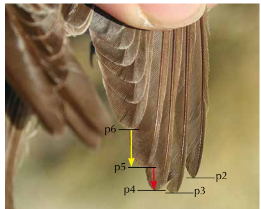
FIGURE 1 Wing-formula of Spotted Flycatcher / Grauue Vliegenvanger Muscicapa striata , Tyrrhenian Flycatcher / Tyrrhense Vliegenvanger M tyrrhenica tyrrhenica and Balearic Flycatcher / Balearische Vliegenvanger M t balearica (Lorenzo Starnini). Note longer distance between tips of p4 and p5 (red) and tips of p5 and p6 (yellow) in Spotted (wing-tip = p3) compared with both Tyrrhenian and Balearic, in which, particularly in latter, distance between these primary tips is shorter. Differences in position of p2 relative to p3 and p5 were already described by Viganò et al (2019). 332 Spotted Flycatcher / Grauue Vliegenvanger Muscicapa striata , adult, Falsterbo, Skåne, Sweden, 22 August 2015 (Marc Illa). Note long distance between tips of p4 and p5 and tips of p5 and p6, with wing-point at p3 (slightly longer than p4) and long p2.
