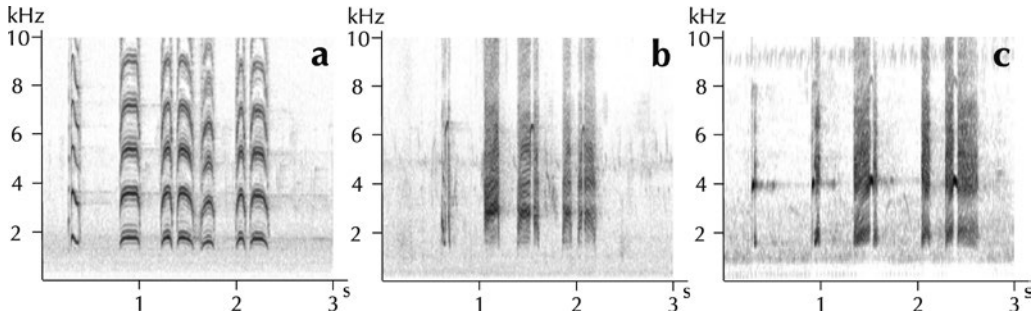
FIGURE 4 Advertising calls compared (www.xeno-canto.org). Black Francolin / Zwarte Frankolijn Francolinus francolinus : a western group (repeated from figure 2a), b eastern group (repeated from figure 3a); Painted Francolin / Bonte Frankolijn F pictus : c XC105864, India ( Vir Joshi )
