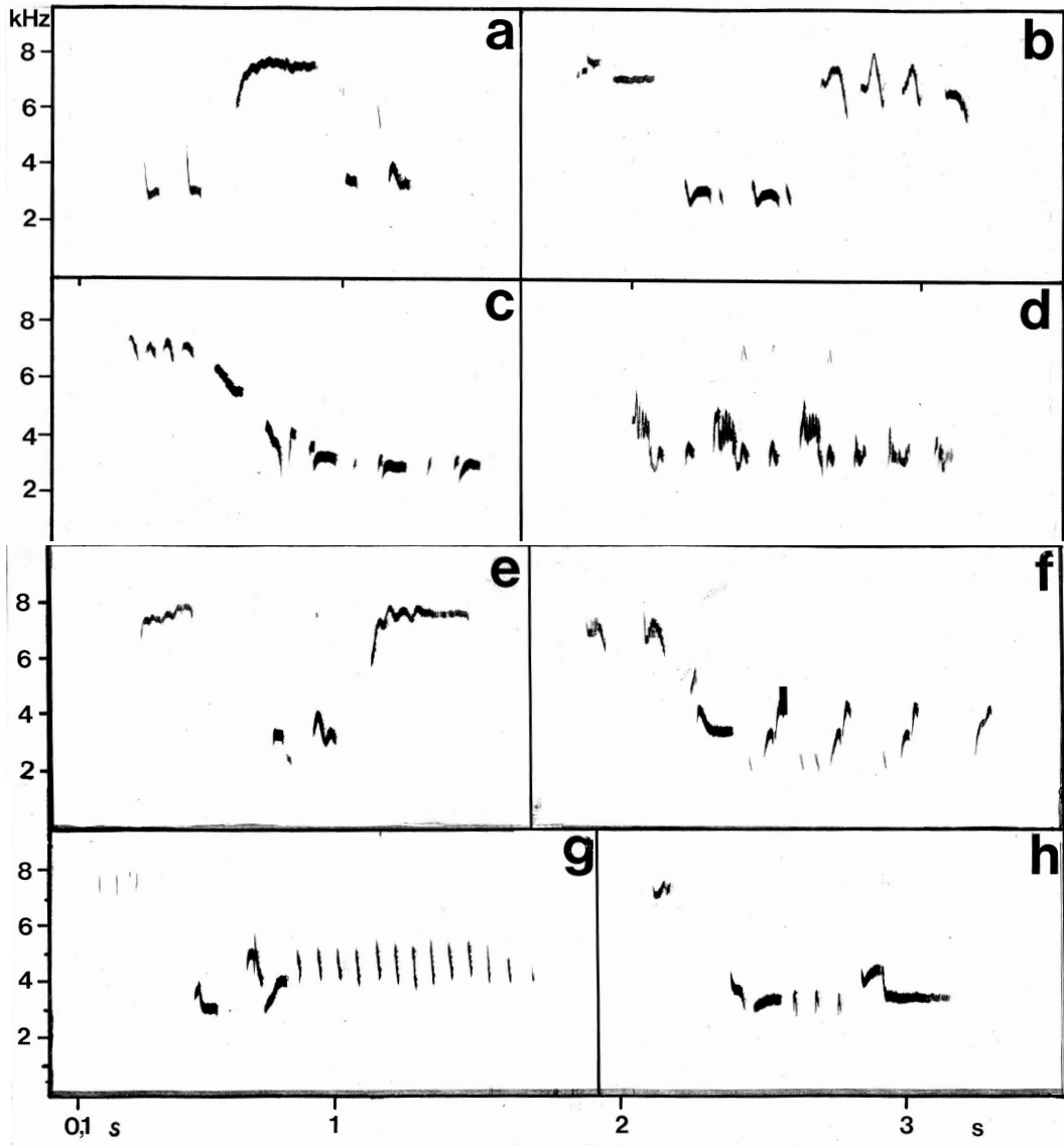
FIGURE 4 Sonagrams of songs of Tenerife Robin / Tenerife roodborst Erithacus superbis , Monte del Agua, Teno mountains, Tenerife, Canary Islands, 20 February 1987 (Hans-Heiner Bergmann). Note rich structure
