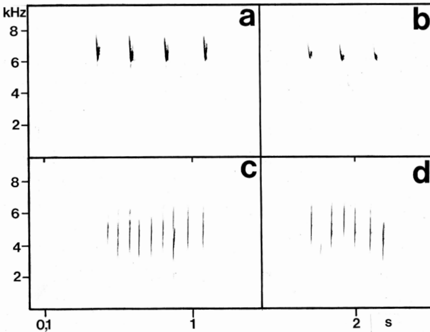
FIGURE 3 Sonagrams of alarm calls of Tenerife Robin / Teneriferoodborst Erithacus superbus and European Robin / Roodborst E. rubecula (Hans-Heiner Bergmann). a-b, Tenerife Robin, Monte del Agua, Teno mountains, Tenerife, Canary Islands, 20 February 1987. c-d, European Robin, Marburg, Hessen, Germany, 16 July 1978
