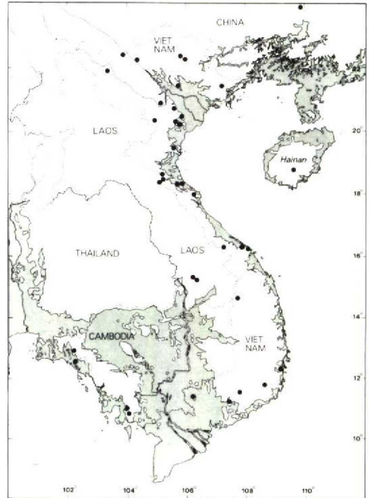
FIGURE 1 Geographical distribution of Blue-rumped Pitta Pitta soror (specimen records and my observations only). Darker shaded area denotes land under 100 m above mean sea level; paler shading indicates coastal waters with depth of less than 50 m
